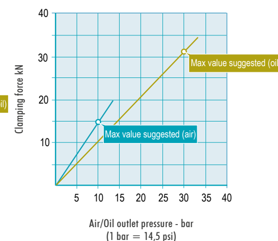
T.3 Hydraulic cylinder Ø135mm Effective surface 132,3mm 2
