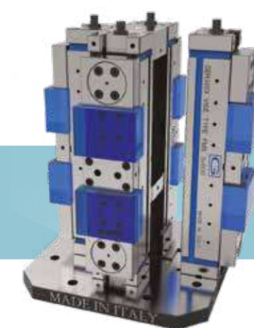
FMS vise tower made of 4 vises Art.865 vertical-mounted through spacers with floating movable jaws and intermediate fixed jaw.
