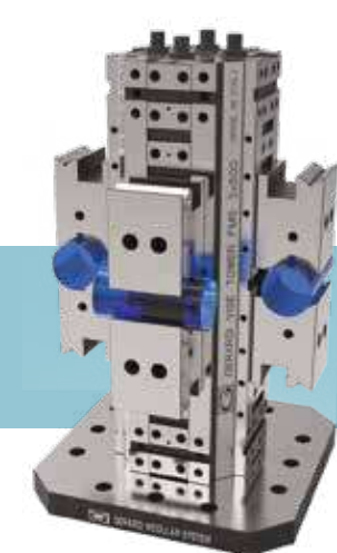
FMS integral vise cube with prismatic movable jaws. Most compact design.
