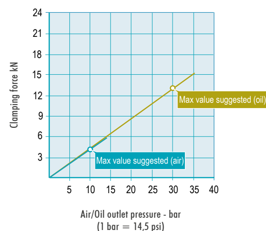
T.2 Hydraulic cylinder Ø85mm Effective surface 51,8mm 2
