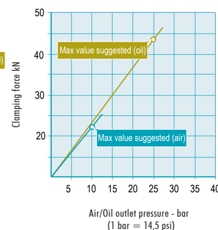
T.4 Hydraulic cylinder Ø170mm Effective surface 209,5mm 2
