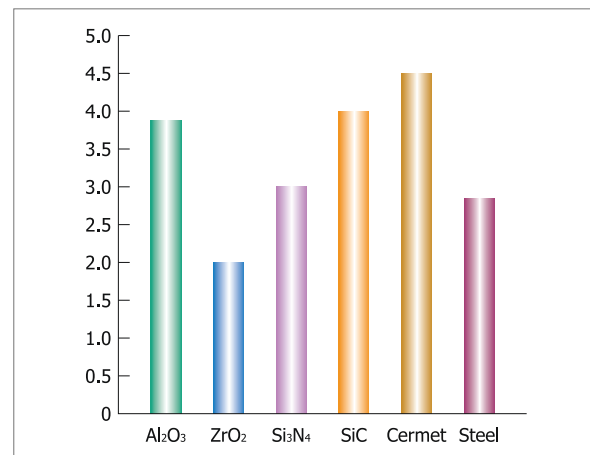
YOUNG'S MODULS (10 6 kg/cm 2 )
