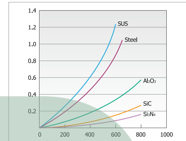
THERMAL EXPANSION (%)
