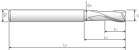
2 FLUTE, DIAMOND COATING END MILL
