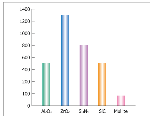
BENDING STRENGTH(MPa)
